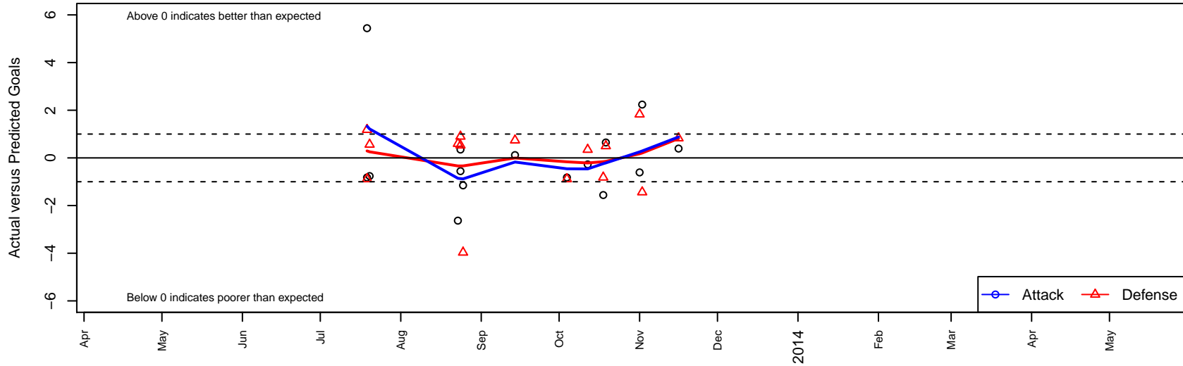
Placer United 01 Red B00 Dots are actual minus expected GF (blue circles) and GA (red triangles). Blue line is smoothed change in attack strength. Red is smoothed change in defense strength.
